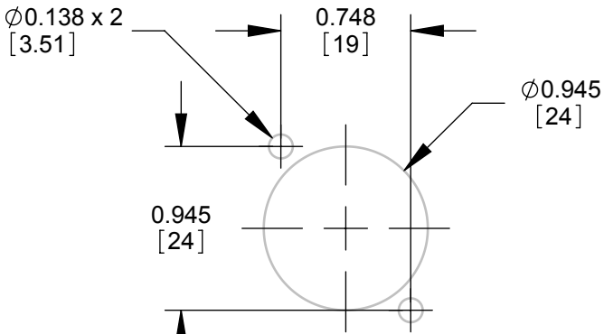
FIGURE 1 RECOMMENDED PANEL CUT-OUT (SCALE 1:1)
